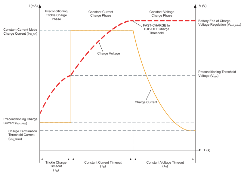
Figure 3: Current vs. Voltage and Charger Time Profile.
